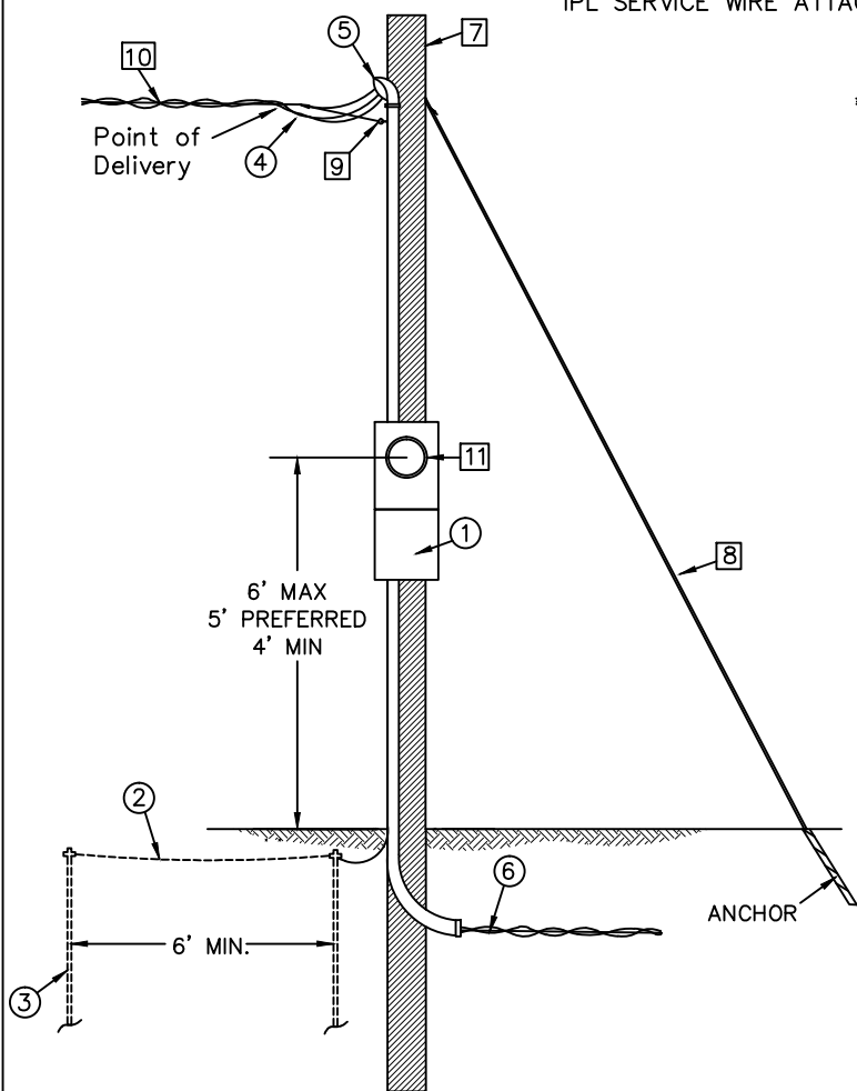
OVERHEAD-UNDERGROUND
